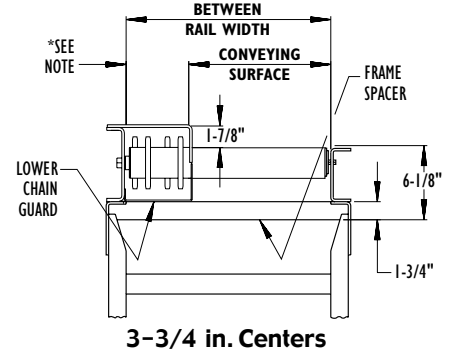
3 in. Centers (Welded Frame)
